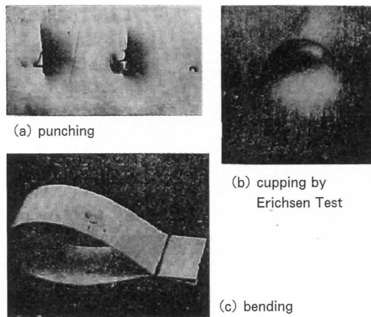
Fig. 3 Test procedure of stress corrosion (season cracking) devised by Igarashi and Kitahara.
