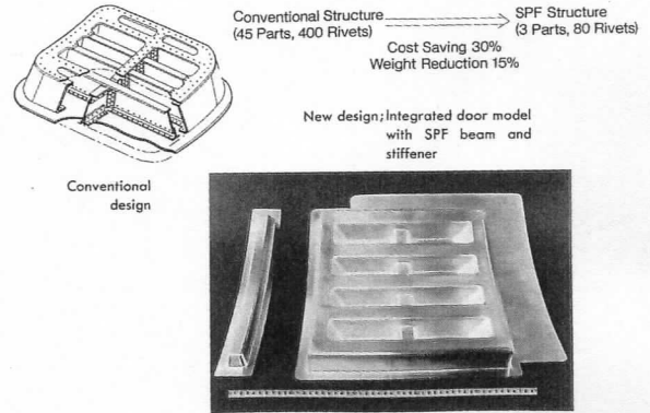
Fig. 8 Integrated door with beam and stiffener deformed by superplastic forming compared to a conventional structure.
