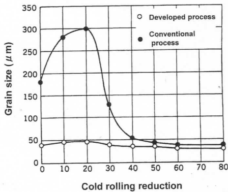
Fig. 7 Effect of the cold rolling reduction on the grain size of stringer produced by newly developed and conventional processes.
