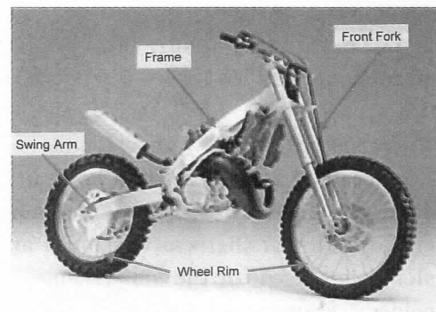
Fig. 12 Motorcycle parts using high strength wrought aluminum alloys for a motocross.
