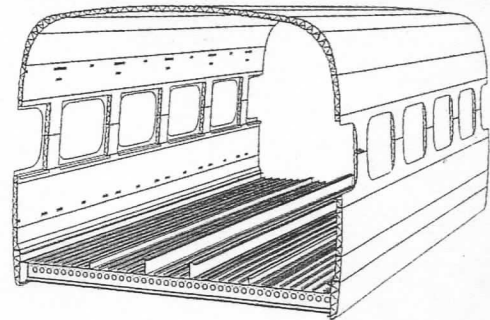
Fig. 11 Series 700 Shinkansen and its body structure produced by 6N01 hollow extrusions with truss cross sections.
