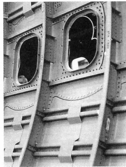
Fig. 5 Fuselage of the Boeing 767.
