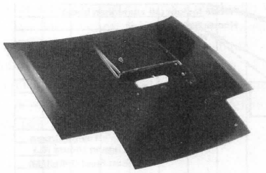
Fig. 14 Aluminum Hood of Mazda RX-7.
