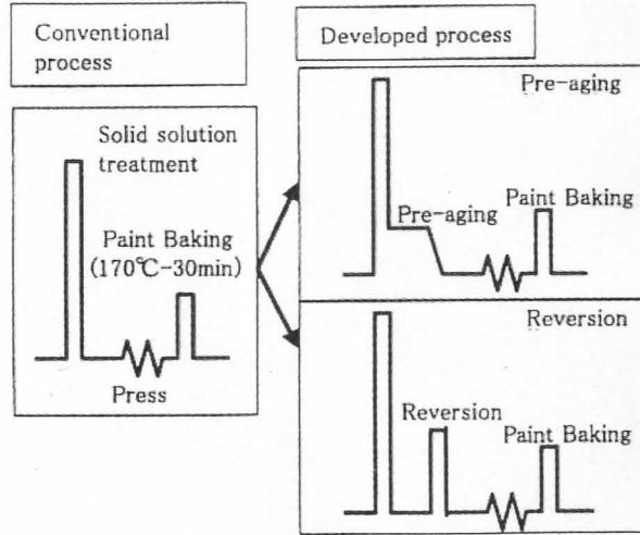
Fig. 15 New processes containing pre-aging or reversion developed for enhancement of bake hardening at 170° .
