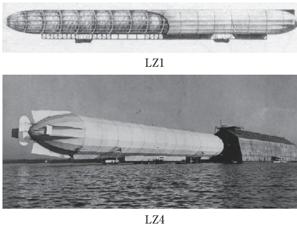
Fig. 4 Structure with gas bags of Zeppelin Airship, LZ1 (top), and LZ4 just before takeoff from the hangar on Bodensee near Friedrichshafen (bottom) 21) . (LZ : works number of Zeppelin, L: Navy's Designation)
