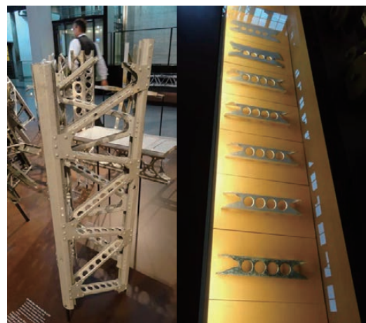
Fig. 5 Part of the Zeppelin airship frame (left) and roll forming process of the frame (right) (Photographed by the author at Zeppelin museum in Friedrichshafen)
