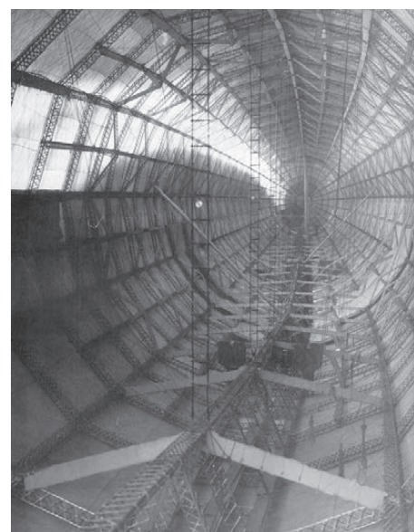
Fig. 6 Inside the hull of the L30 (LZ62), looking forward, after application of the outer cover, but before the gas cells were in place 21) .
