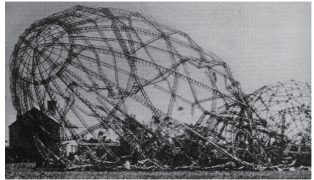
Fig. 7 The skeleton of L33 (LZ76) by New Hall Cottages, little Wigborough, Essex. There was so little hydrogen left in the gas cells that the attempt to destroy the ship by fire left the framework almost intact, providing a useful source for the British authorities 22) .
