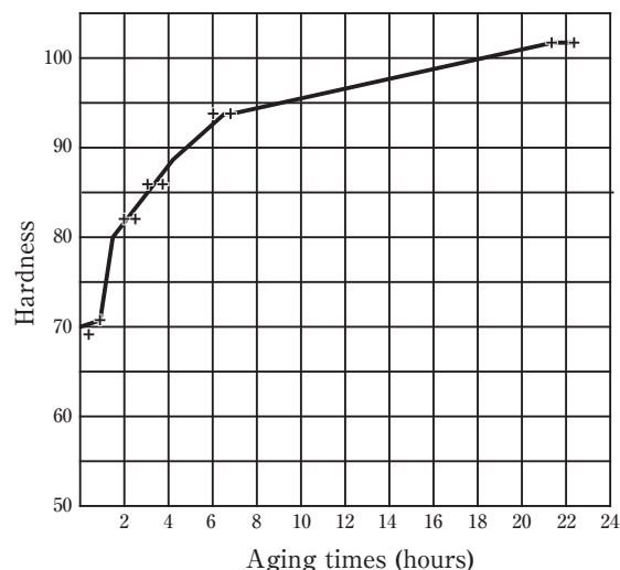
Fig. 10 Age hardening at room temperature in Al-3.5%Cu-0.5%Mg alloy published by A. Wilm (Vertical axis: hardness, Horizontal axis: aging times (hours)) 25) .
